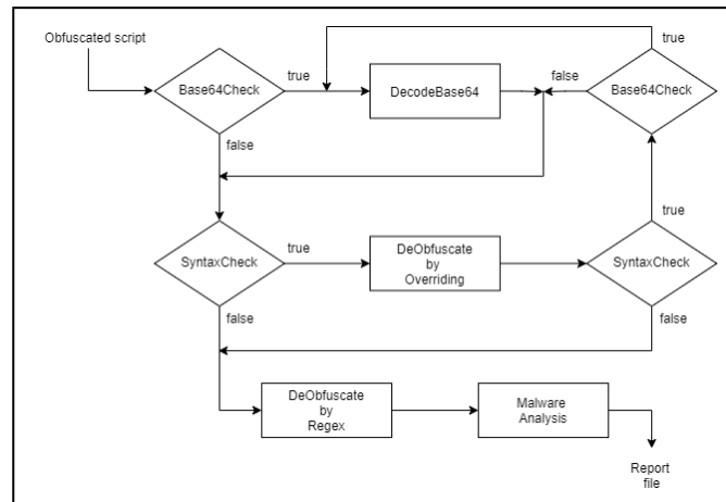
Figure 1: PowerDecode operation scheme
